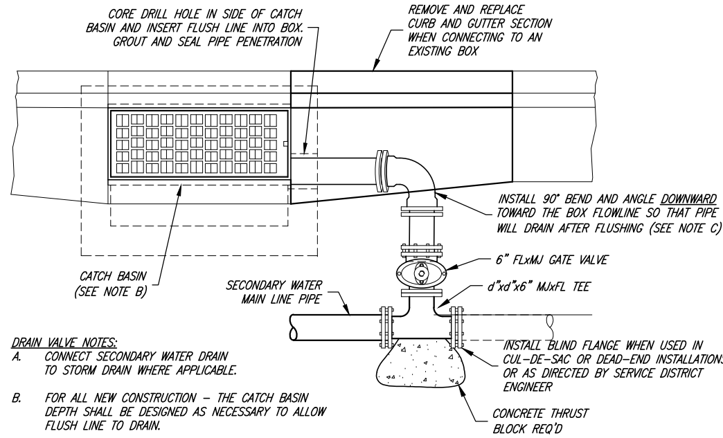
TYPICAL DRAIN VALVE DETAIL
