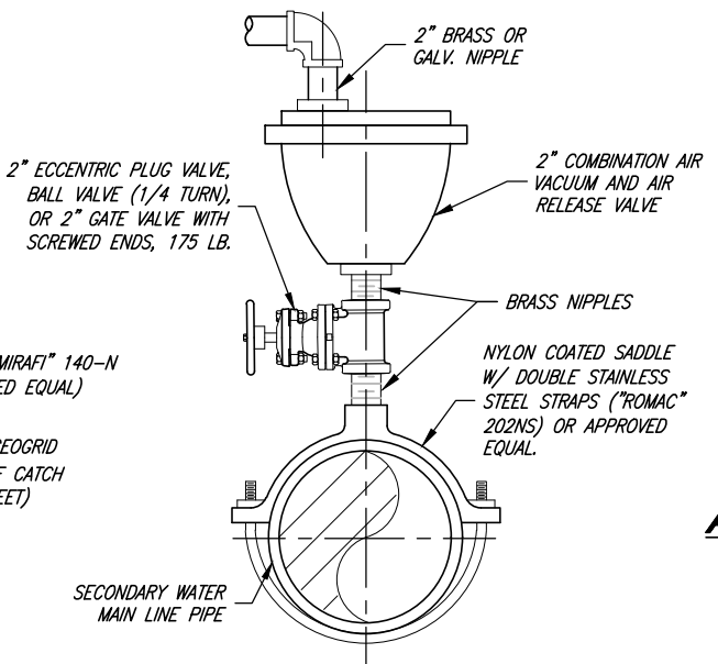
AIR-VACUUM AND AIR-RELEASE VALVE
