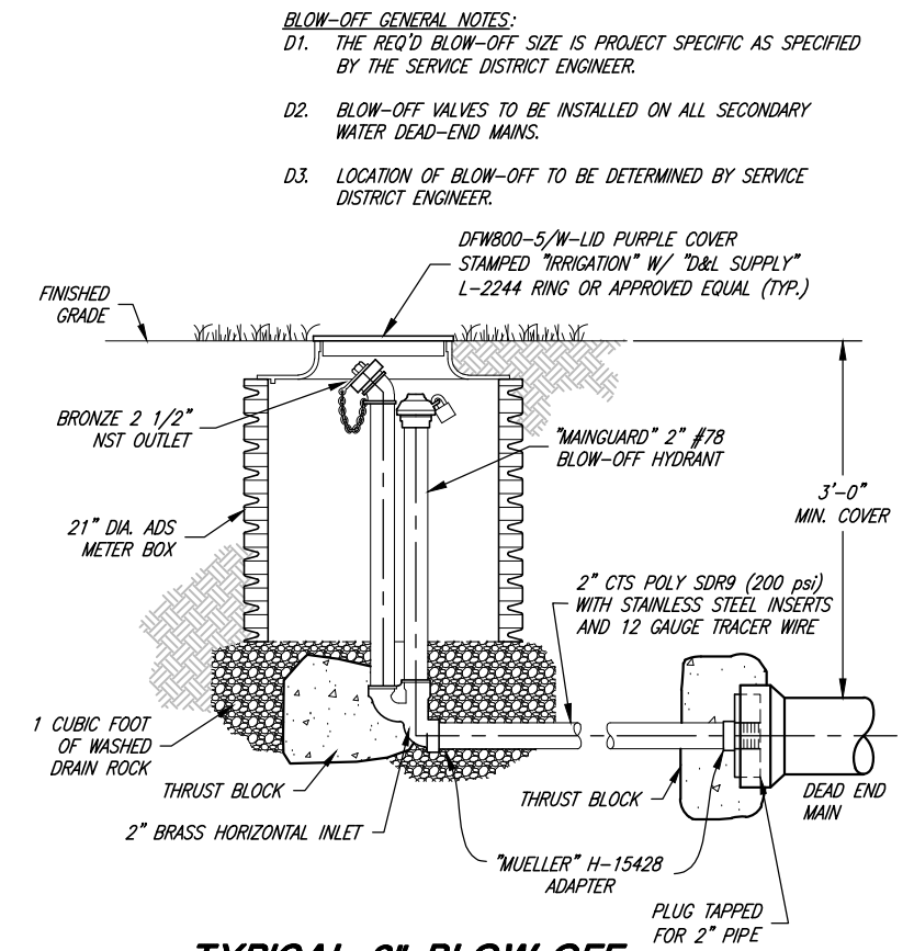
TYPICAL 2" BLOW-OFF (FLUSH) VALVE CONNECTION
