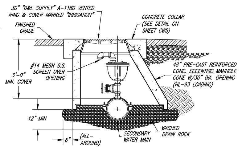
AIR VACUUM & AIR RELEASE VALVE STREET INSTALLATION
